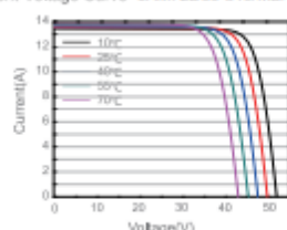
Current-Voltage Curve JAM72D30-540/MB/1500V
